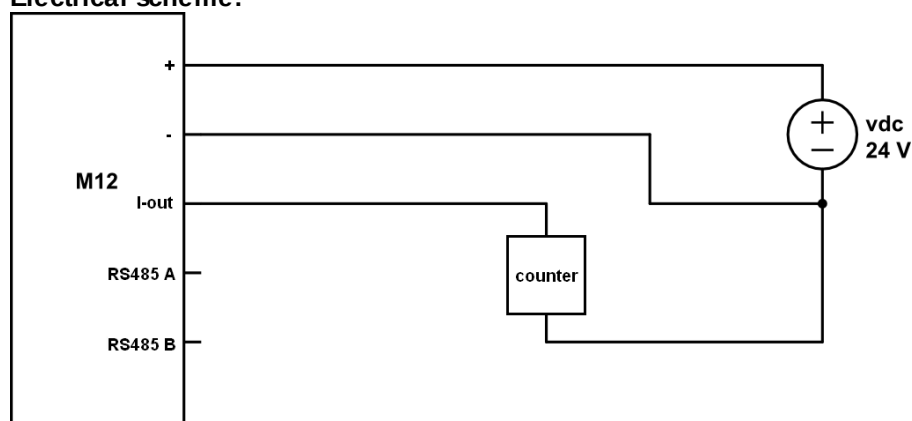
Electrical scheme:
