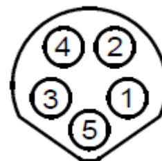
M8 5-pin female connector
